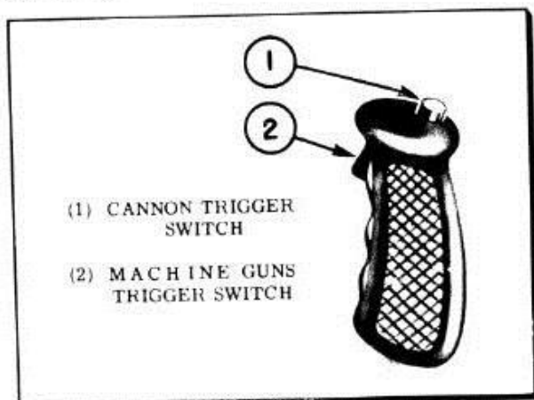
Figure 3 - Control Stick Grip
