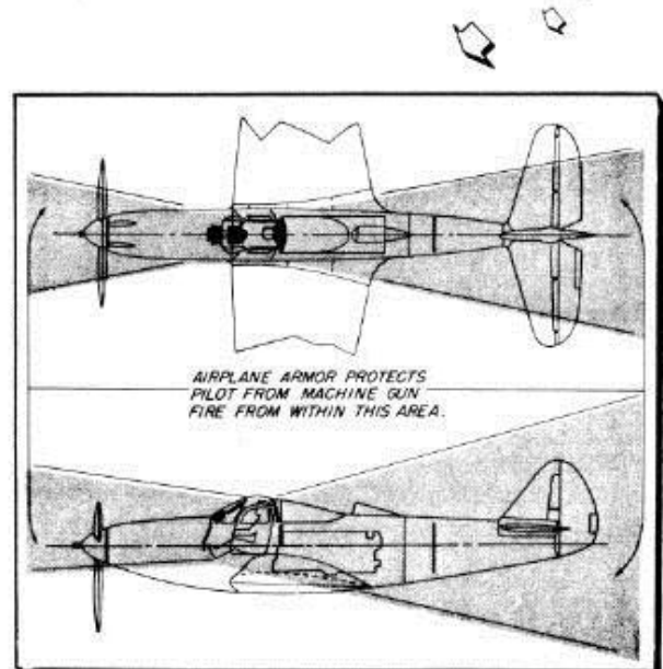
Figure 2 - Armor Plate
