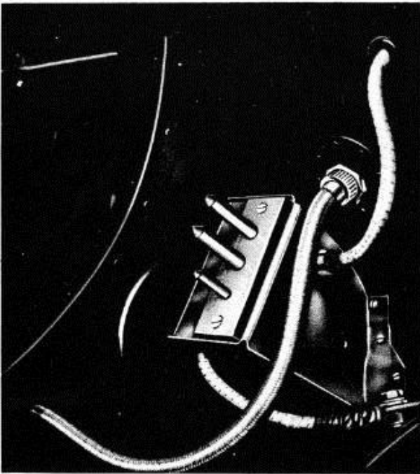
Figure 16 - Plug - External Power Source
