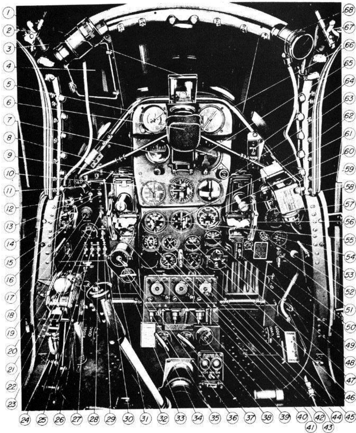
Figure 5 - Cockpit - Front View
